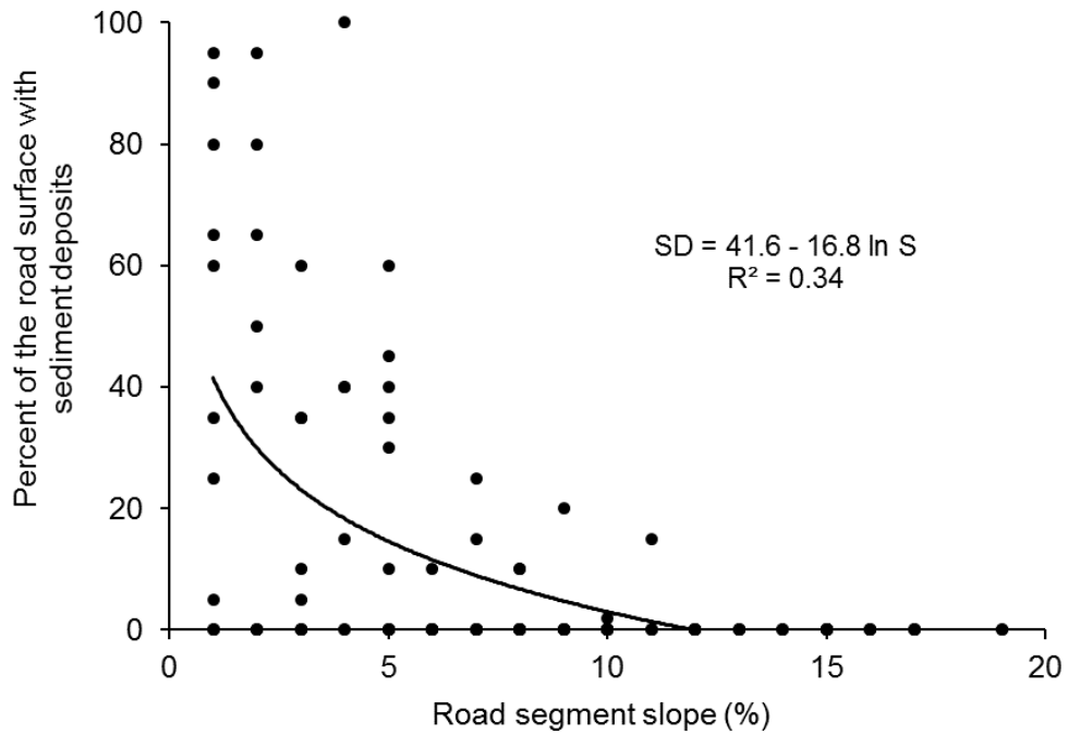
Figure 1.8. Percent of the road surface with sediment deposits (SD) versus road segment slope (S).
