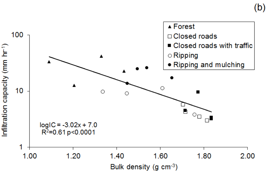
Figure 2.10. Relationship between the log-transformed infiltration capacity and (a) ground cover, and (b) bulk density for all 20 rainfall simulations.
