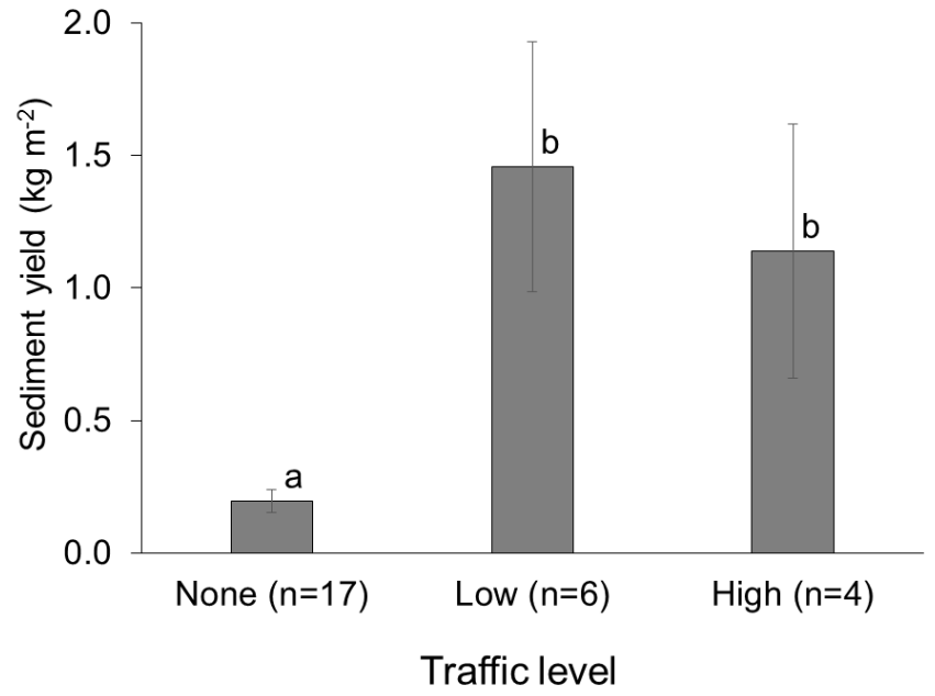
Figure 3.6. Sediment production by traffic level for the first period of summer 2013. Error bars are the standard error, and different letters indicate significant differences.
