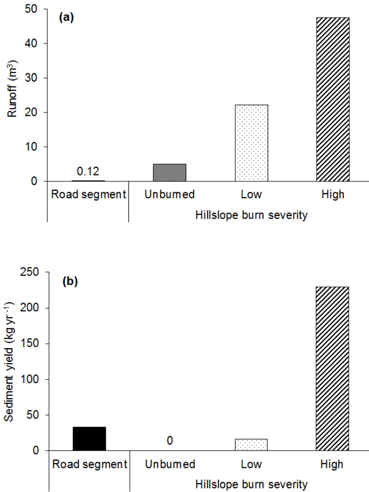
Figure 1.12. Comparison of the (a) predicted surface runoff (m 3 ) and (b) predicted sediment yields (kg yr -1 ) from an average road segment using WEPP:Road and an unburned, low severity, and high severity hillslope above the road using Disturbed WEPP. The modeled hillslope used the mean values for hillslope length, slope, and soil type.
