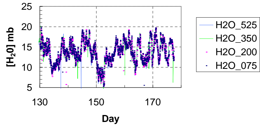
Combretum H 2 O Profile
