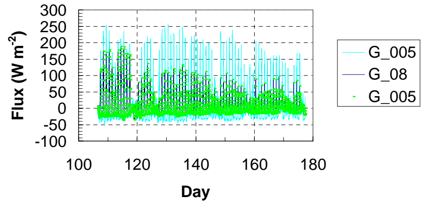
Near Surface Soil Heat Flux
