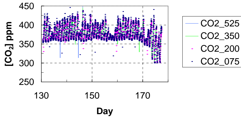
Combretum CO 2 Profile
