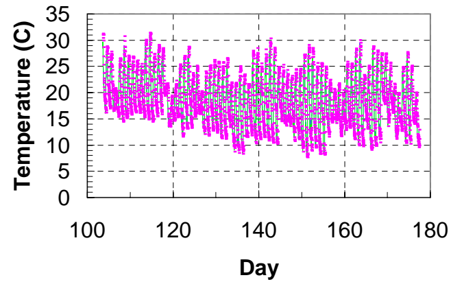
Air Temperature Profile
