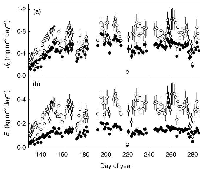
Fig. 3. (a) Whole-tree water flux per unit sapwood area ( J_s , \text{mg m}^{-2} \text{ day}^{-1} ) in 10 m (○) and 25 m trees (●). Bars represent standard errors. J_s is the weighted average of both outer (0–10 mm beneath cambium) and inner (10–30+ mm beneath cambium) sap flux densities. (b) Whole-tree water flux per unit leaf area ( E_L , \text{kg m}^{-2} \text{ day}^{-1} ).
