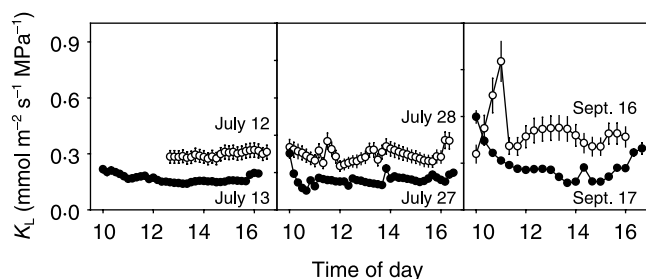
Fig. 2. Whole-tree leaf-specific hydraulic conductance ( K_L , \text{mmol m}^{-2} \text{s}^{-1} \text{MPa}^{-1} ) for 10 m ( \circ ) and 25 m trees ( \bullet ) during three diurnal courses from mid- to late season 1999. Standard error bars are not visible on all points.
