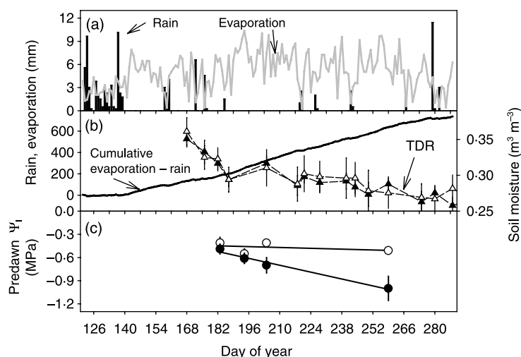
Fig. 1. (a) Rainfall and pan evaporation near the plots. (b) Cumulative evaporation minus rainfall, and soil moisture (with standard error bars) averaged from five locations under the 10 m ( \Delta ) and the 25 m trees ( \blacktriangle ). (c). Predawn leaf water potentials measured from 10 m ( \circ ) and 25 m trees ( \bullet ). Standard error bars are not visible on all points.
